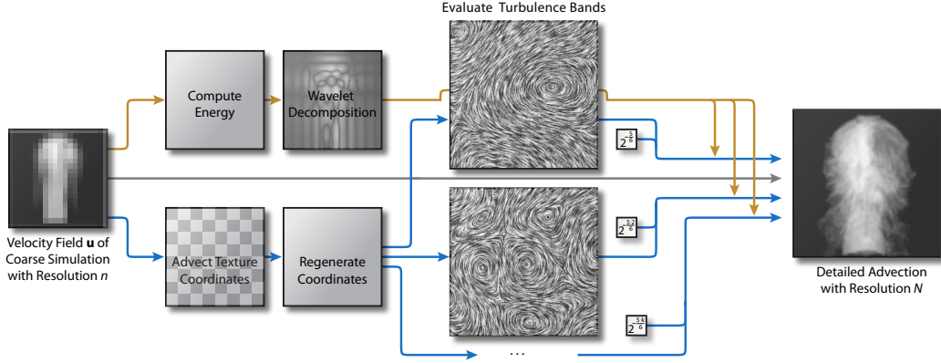
Figure 2: Overview: A low-resolution n^3 velocity field \mathbf{u} is used to synthesize a high-resolution N^3 density field. Procedural turbulence is added according to the wavelet decomposition of the energy, and the resulting eddies are advected via texture coordinates until they scatter.
